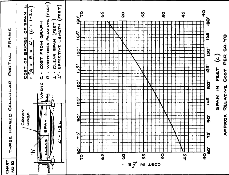
Fig. 262.—Cost of Three-hinged Portal-frame Bridges.
